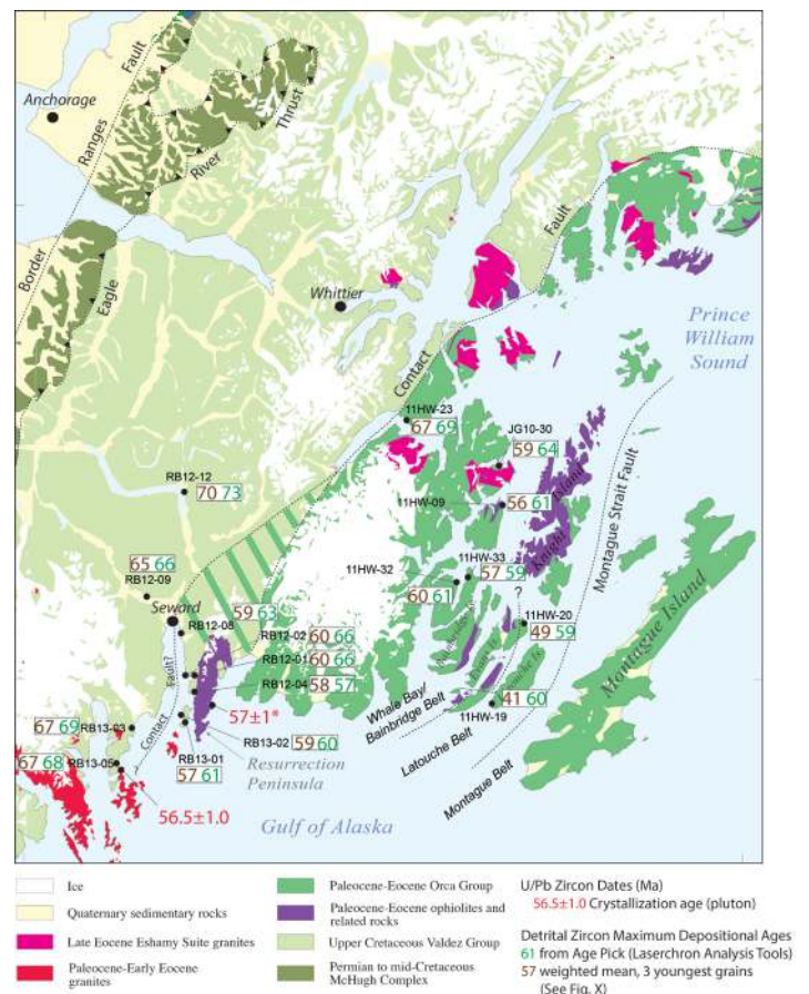
Figure 1. Geologic map and sample locations from the Chugach-Prince William Terrane in western Prince William Sound, Alaska. Modified from Bradley (2006) and Kveton (1989). U/Pb zircon crystallization ages of plutons shown in red, and maximum depositional ages from detrital zircon samples also shown (see key). *from Bradley and Miller, 2006.
