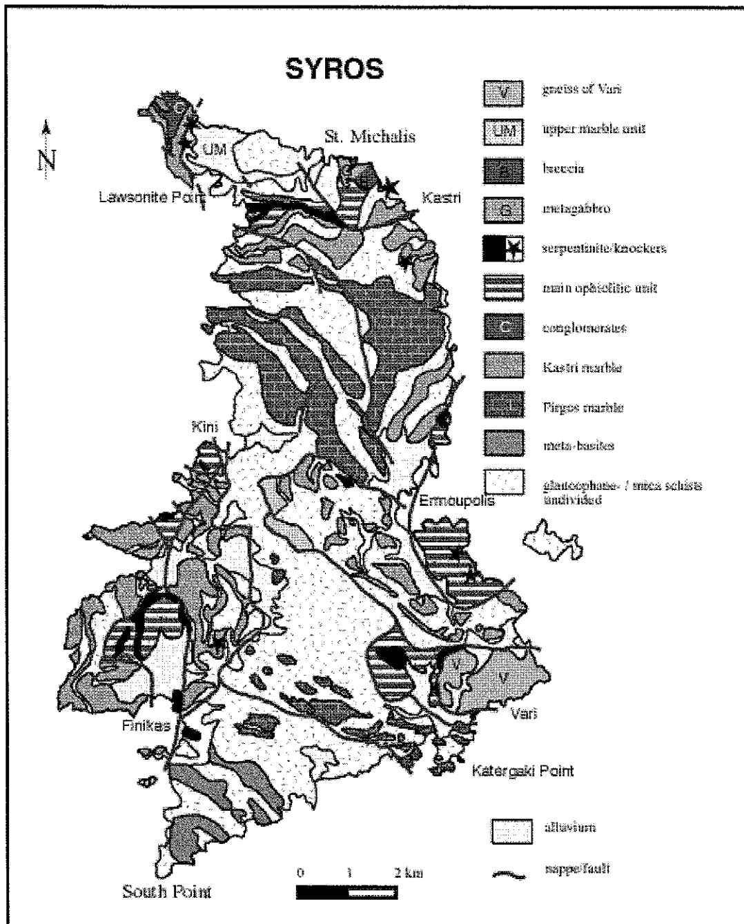
Figure 2. Generalized Geology of Syros modified from Höpfer and Schumacher (1997)
