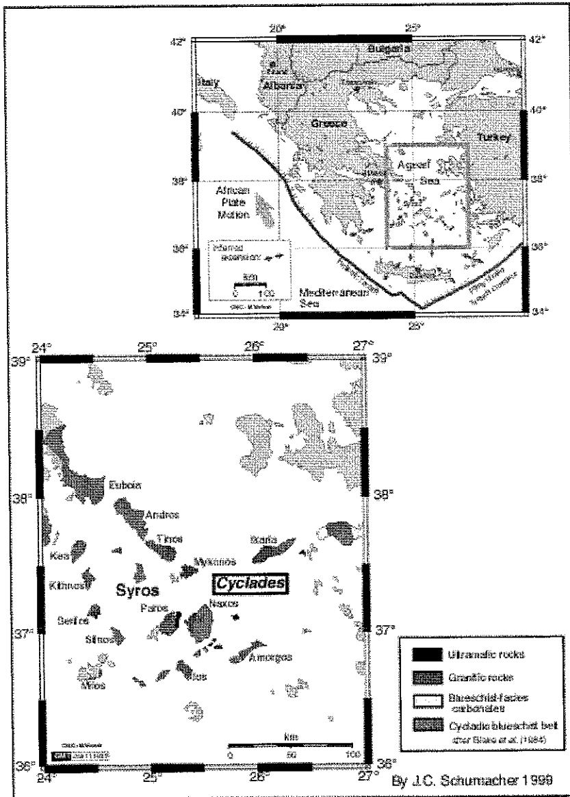
Figure 1. Tectonic map of the Aegean Sea with the location of Syros and the Cycladic Islands (top) and the important rock types in the Attic-Cycladic complex (bottom).
