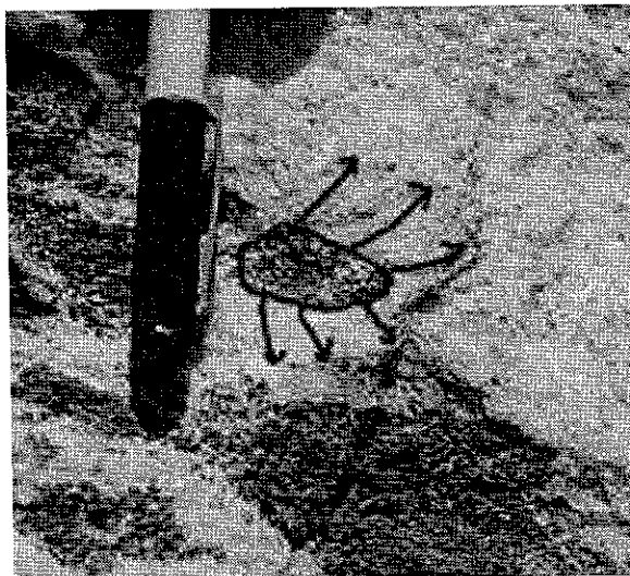
Figure 4. Two centimeter garnet boudin surrounded by calcite needles which fan completely around the structure. Pen for scale.
