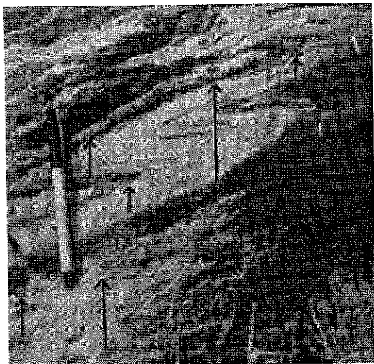
Figure 5. An isoclinal folded impure marble layer. The calcite needles sweep across the fold and remain sub-perpendicular to foliation. Pen for scale.
