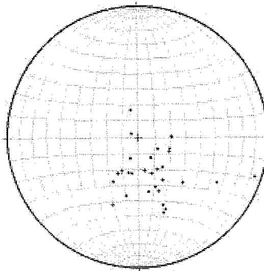
Figure 2. Poles to foliation across Syros.
