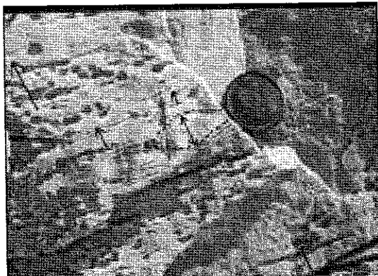
Figure 3. A clast of pure calcite needles in a marble matrix. The needles in the boudin are parallel to the surrounding matrix needles, which are sub-perpendicular to foliation. Lens cap for scale.
