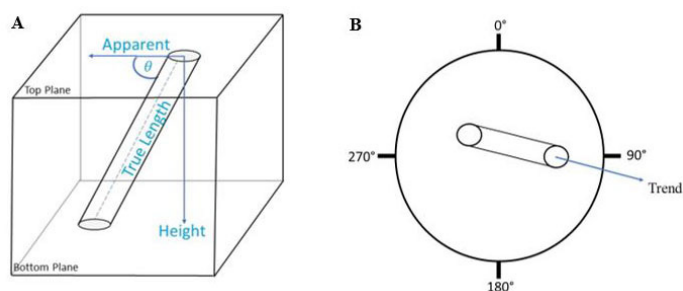
Figure 1. Schematic diagram illustrating characterization of microlite orientation through trend ( \phi ) and plunge ( \theta ), adapted from Castro et al. (2002). A: 3D schematic of a microlite between two focal planes. The apparent length measured from the top plane, moving down to the bottom plane to gain the height allows for the plunge ( \theta ) to be calculated. The true length is then derived from the Pythagorean Theorem. B: Goniometer is utilized to determine the trend of the microlite based on its long axis.
