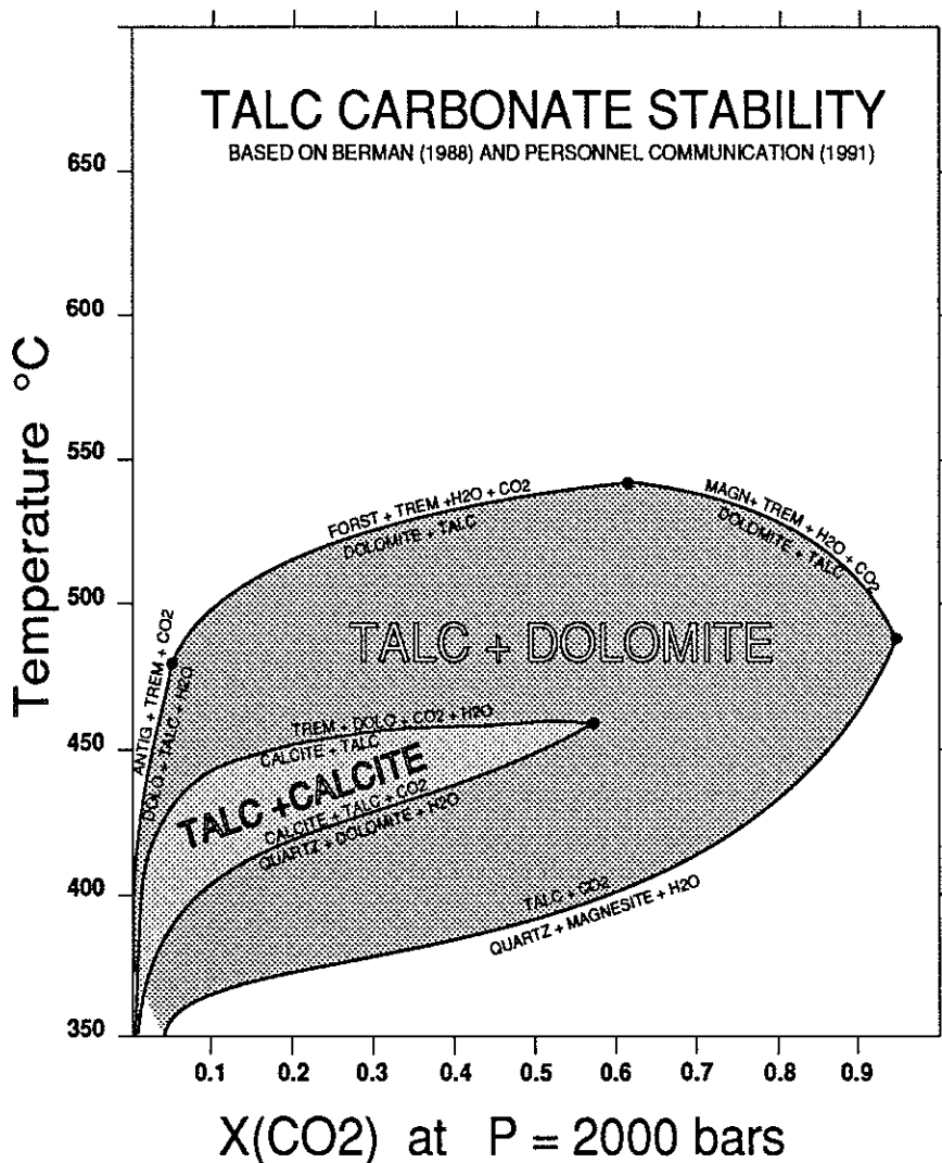
Figure 2. Calculated talc-dolomite and talc-calcite stability relations.
