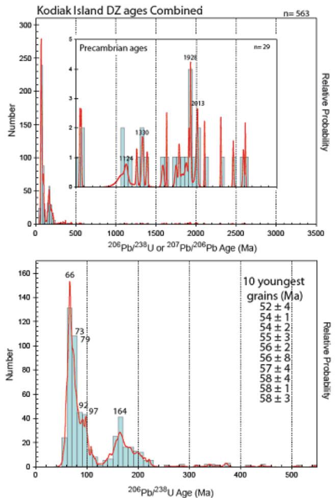
Figure 2: Probability Density plot (red line) and histogram (blue bars) showing age distribution of combined data. Top highlights oldest Precambrian grains ( n=29 ), and bottom shows youngest peaks produced with a list of the 10 youngest grains collected. Figure by Hannah Hilbert-Wolf.
