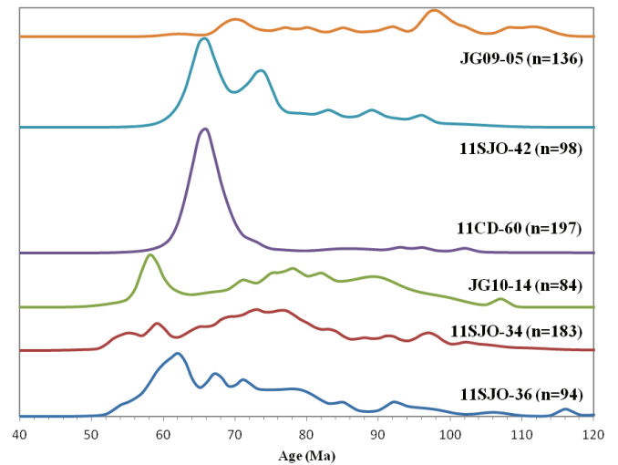
Figure 3: Grain age distribution of all zircon analyzed in this study. These units were individually mixed to produce an estimate for the sedimentary provenance of the middle Miocene Narrow Cape Formation. Relative probability on the y-axis.
