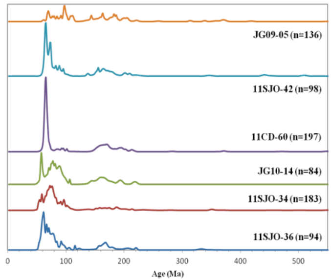
Figure 4: Probability Density plot versus age of selected DZ age distributions (oldest sample top to youngest sample bottom). Top shows ages in the Phanerozoic.
